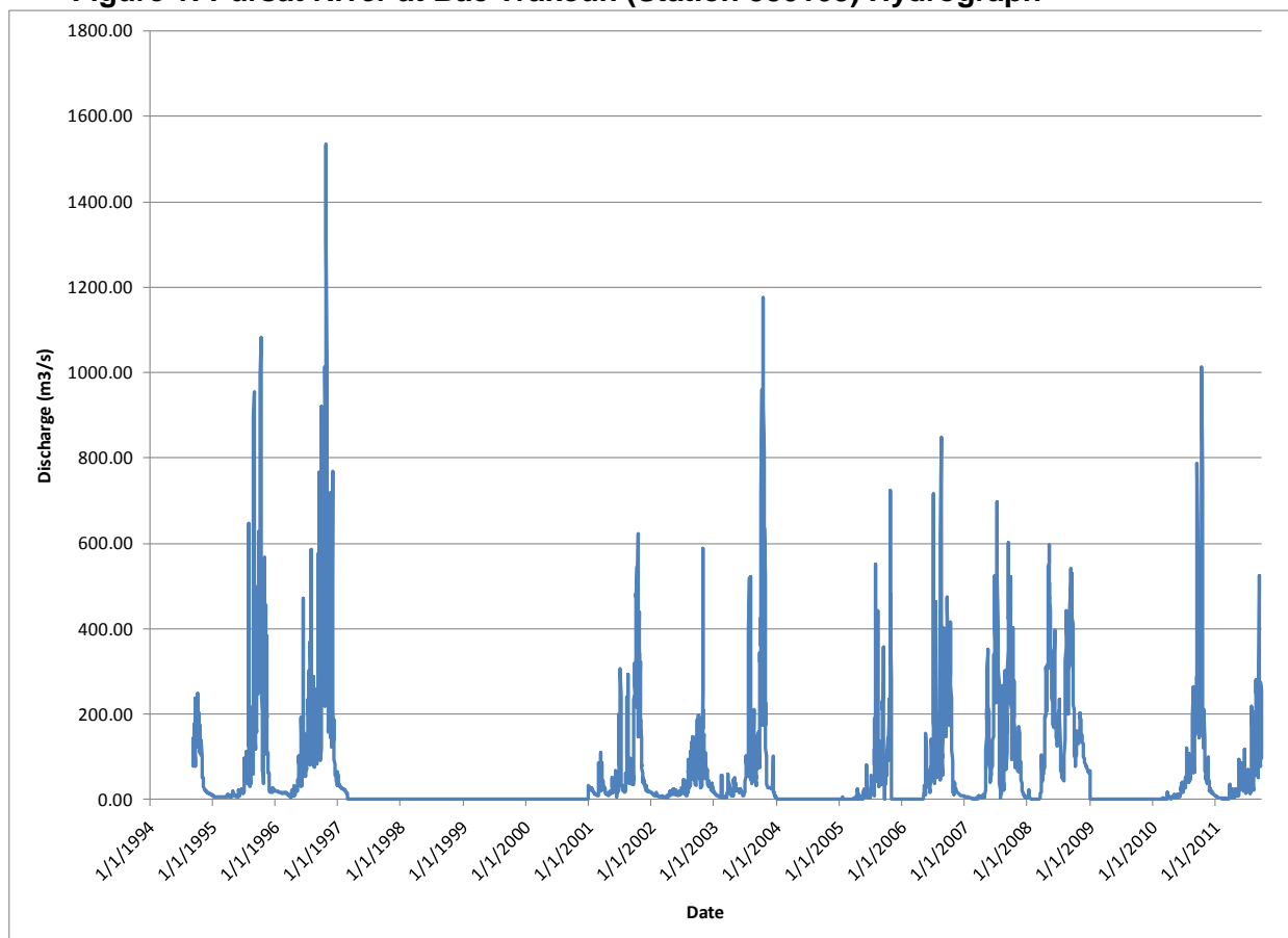
Figure 1: Pursat River at Bac Trakoun (Station 580103) Hydrograph
