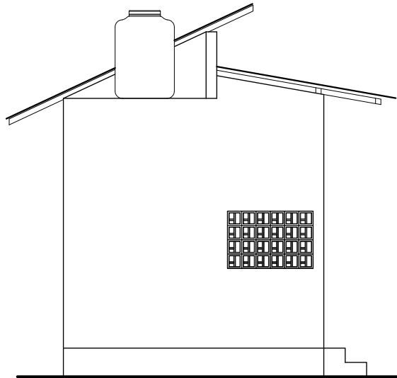
TAMPAK SAMPING KIRI Skala 1 : 75
