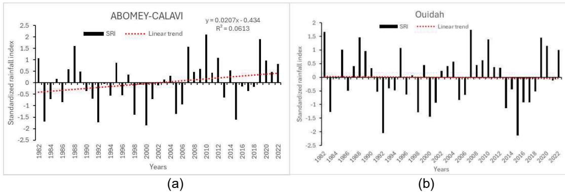
Figure 1: 1982–2022 Standardized Precipitation Index for Abomey-Calavi and Ouidah (Atlantique Department)
