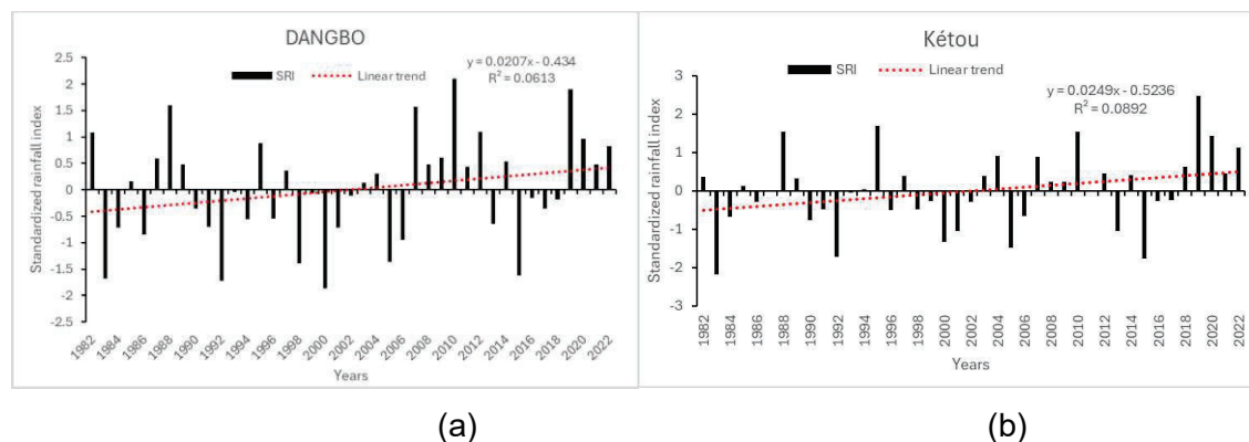
Figure 2: 1982–2022 Standardized Precipitation Index for Dangbo (Ouémé department) and Kétou (Plateau department)
