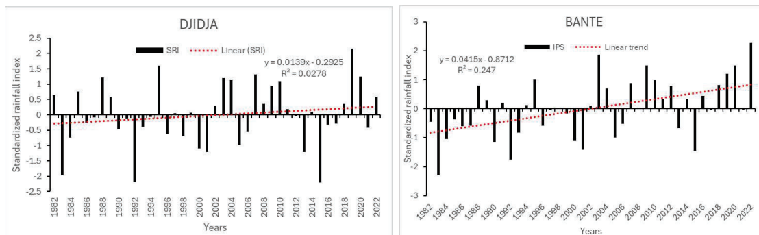
Figure 4: 1982–2022 Standardized Precipitation Index for Djidja (Abomey department) and Bantè (Collines department) Source: METEO BENIN, 2025.
