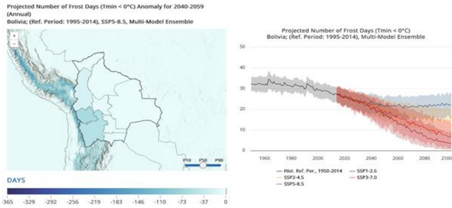
Figure 5: Trend in the annual number of frost days ( <0^{\circ}\text{C} , 2050) with the SSP5-8.5 scenario (left) and projections with all scenarios (right) in Bolivia. Sources: World Bank CCKP.
