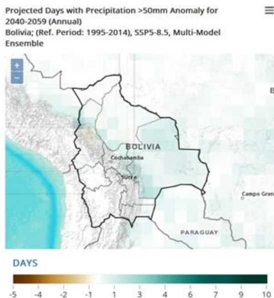
Figure 8: Trend in the annual number of days with precipitation >50mm (2050) with the SSP5-8.5 scenario in Bolivia. Sources: World Bank CCKP.
