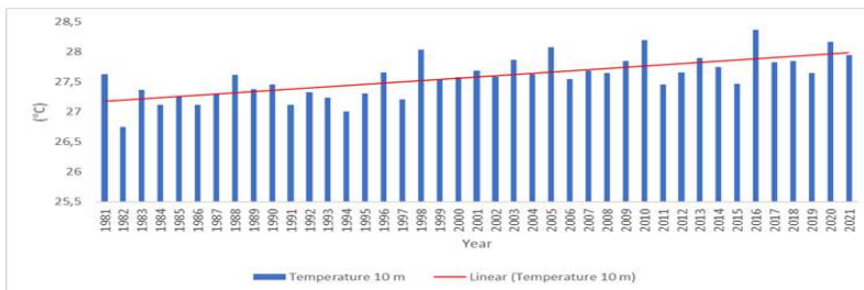
Figure 2. Temperature Trends Period 1981-2021
